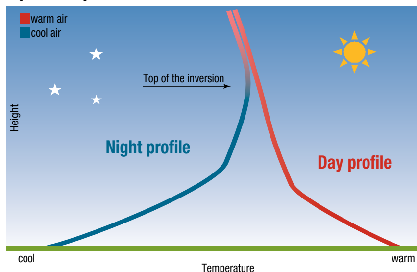
FIGURE 1: Typical vertical temperature profiles for a point in time during the night and day. At low levels, the day profile typically cools with height and the night profile typically warms with height. Little change occurs at elevated altitudes.
